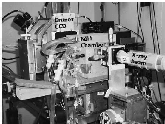
Fig. 10. Physical setup at D1 station at CHESS.
