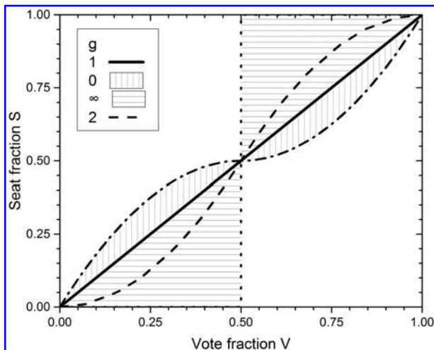
FIG. 2. Ideal (zero bias) seats-votes possibilities for four voter-centric measures identified by the values of g .
