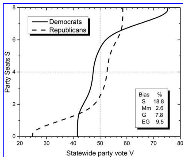
FIG. 4. Seats vs. votes curves for Maryland 2012 congressional election. The lower right legend gives values of bias for four different methods discussed in the text.
