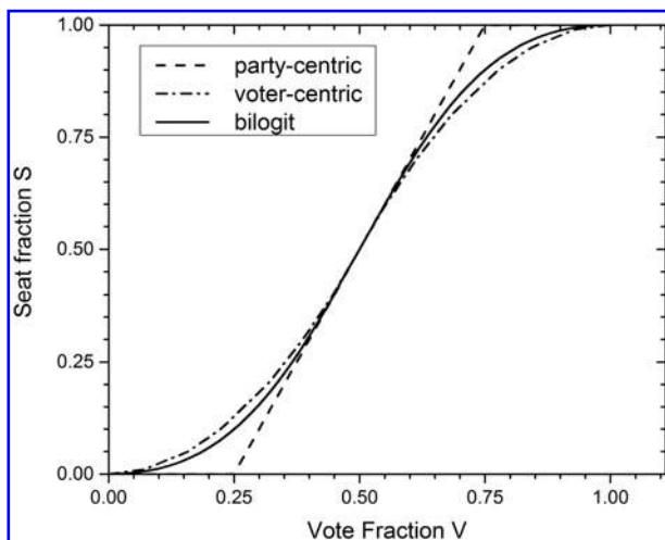
FIG. 3. Comparison of three S(V) functions with the same level of responsiveness R=2 .
