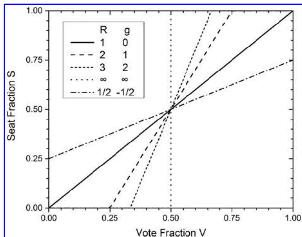
FIG. 1. The solid line shows zero bias for proportional representation, and the long dashed line shows zero bias when equalizing wasted votes. Other zero bias functions with other values of responsiveness R are the seats-votes functions S_g(V) for the party-centric fairness criterion given by Eq. (1).
