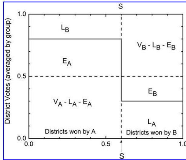
FIG. B1. Illustration of basic average quantities. The district votes have been averaged within each group of districts won by voters of like mind.
