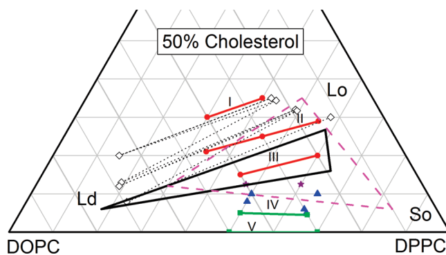
Figure 7. NMR tie-lines of VSKG 18 are shown by dotted straight lines, and open diamonds show end points at the two-phase Ld–Lo boundary. The Ld–Lo–So three-phase region is shown as a solid black triangle, 18 and the dashed magenta triangle is the three-phase region from DCJ. 19 As in Figure 2, the orientations (not the end points) of our tie-lines are labeled I–V. The red circles and the green squares are in two-phase regions, the blue triangles are in a three-phase region, and the purple stars could be in either two-phase or three-phase regions. All results are for T = 15^\circ\text{C} except for T = 18^\circ\text{C} for the three-phase triangle of DCJ. 19
