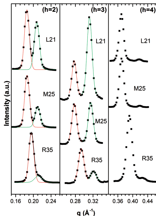
Figure 1. Lamellar peak data (squares) versus q for orders h = 2 – 4 for three samples, L21, M25, and R35. Green and red lines are Gaussian fits, and uncertainties in their peak positions correspond to 0.2 Å uncertainties in D -spacings.
