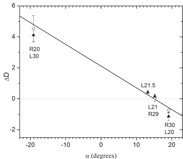
Figure 5. Differences \Delta D between curves of the double D -spacing data in Figures 3 and 4 relative to the M25 data as a function of \alpha which is the angle of the lines passing through M25 in Figure 2. Solid symbols are for the L compositions, and open symbols are for the R compositions. The linear fit to all data is shown by the solid line.
