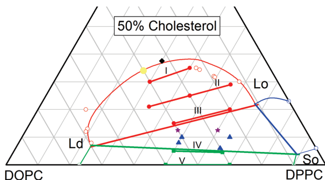
Figure 8. Suggested phase diagram at T = 15\text{ }^{\circ}\text{C} . The Ld-So two-phase region is enclosed by three straight green lines and contains our IV and V tie-line fragments; the two open green circles at zero Chol show the coexistence compositions of Mitsui and Furuya. 30 The Ld-Lo two-phase region is enclosed by one straight and one curved line, and it contains our I, II, and III tie-line fragments; the open red circles show the coexistence compositions of VSKG. 18 The Lo-So two-phase region is enclosed by two straight lines and one curved blue line; the open blue circles at zero DOPC show the coexistence compositions of Vist and Davis. 34 The yellow point suggests the location of an upper consolute (critical) point, and we found only one D -spacing for the composition of the black diamond.
