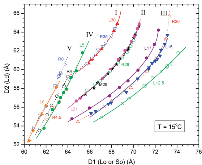
Figure 4. Double D -spacing data that locate tie-lines: I (L30-R35 with \alpha_I = 19.2^\circ ), II (L21-M25-R29 with \alpha_{II} = 15.2^\circ ), III (L15-R20 with \alpha_{III} = 14.1^\circ ), IV (L5-R4.5 with \alpha_{IV} = -2^\circ ), and V (L0-R0 with \alpha_V = 0 ). Solid lines are fits to the L data (solid symbols), and dotted lines are fits to the R data (open symbols).
