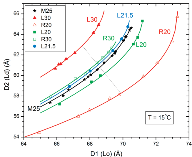
Figure 3. D_2 is the repeat spacing of the Ld phase, and D_1 is the repeat spacing of the Lo phase for many different equilibrated hydration levels for six samples with short names indicated in the legend. Lines are fits of eq 1 to the data. Deviations of individual D values from these lines are consistent with the uncertainties obtained from fitting the data in Figure 1. The different L and R samples are equidistant from the M25 sample in the composition triangle in Figure 2. For quantitative error analysis, average differences between hydration curves along several lines such as the dotted line were used.
