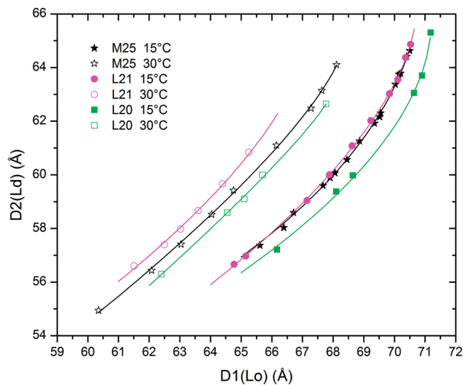
Figure 6. Temperature dependence of the double D -spacing data which show that \alpha_{II} rotates from 15.2^\circ at 15^\circ\text{C} to 17.1^\circ at 30^\circ\text{C} . Data not shown indicate that d\alpha_{II}/dT increases with increasing T .
