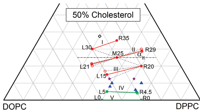
Figure 2. Truncated ternary DOPC/DPPC/Chol Gibbs composition triangle showing compositions of studied samples with some of their short names. Table 1 lists all numerical compositions by name. Circles (red) indicate compositions with Ld-Lo coexistence, squares (green) indicate Ld-So coexistence, triangles (blue) indicate Ld-Lo-So coexistence, stars (purple) could be either in two-phase or in three-phase coexistence, and the open (black) diamond is in a single phase. The solid lines labeled with Roman numerals show the orientations of our best determined tie-lines at T = 15^\circ\text{C} , and the dashed lines show orientations that were determined not to be tie-lines. The ends of the tie-lines were not determined in this study, so the tie-lines shown are partial fragments of the tie-lines that must extend further in both directions.
