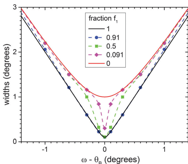
Fig. 6 The widths (FWHM) of the sum of two Lorentzians in eqn (3). The fraction of the total intensity in the first Lorentzian is f_1 . The first Lorentzian was given width w_{M1} = 0.1^\circ and the second Lorentzian was given width w_{M2} = 1.0^\circ .
