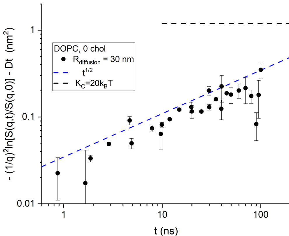
Fig. S4. Time dependence of the MSD assuming the radius for diffusion is 30 nm. The required monotonicity is doubtful, suggesting that diffusion has been over-corrected.
