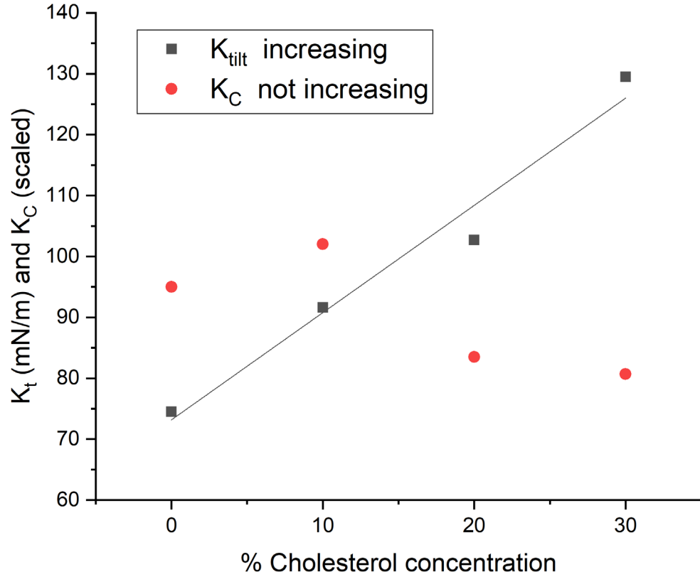
Fig. S3. Result of re-analysis of the original x-ray diffuse scattering data, Pan et al., Phys Rev E 80 (2009) 021931, that includes the tilt modulus K_t as well as the bending modulus K_C using the analysis method of Jablin et al., Phys. Rev. Lett. 113 (2014) 248102. The average K_C/kT was 20 for no cholesterol.
